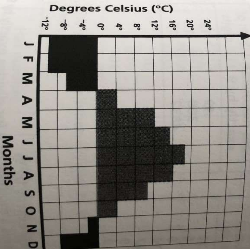
Average monthly temperatures in Moscow
