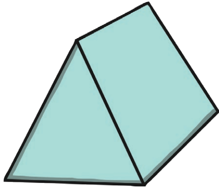
triangular prism
