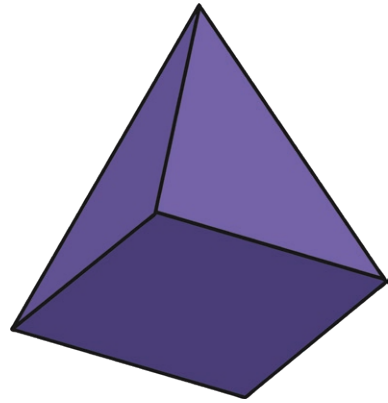
square-based pyramid
