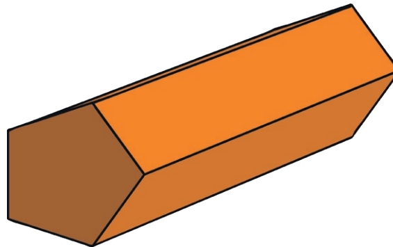
pentagonal prism
