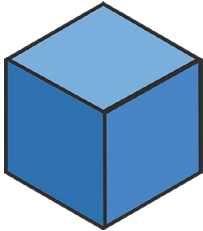
cube
