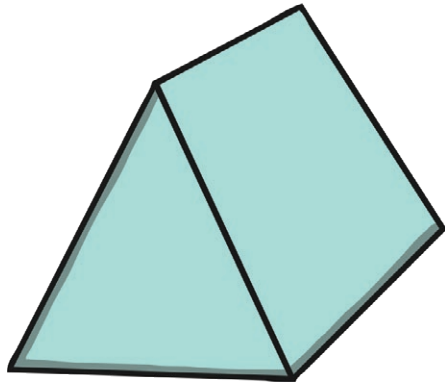
triangular prism
