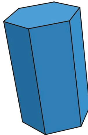
hexagonal prism
