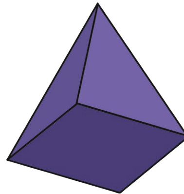
square-based pyramid
