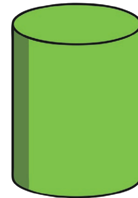
cylinder
