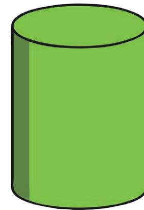
cylinder
