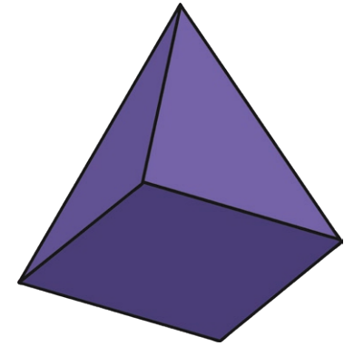
square-based pyramid
