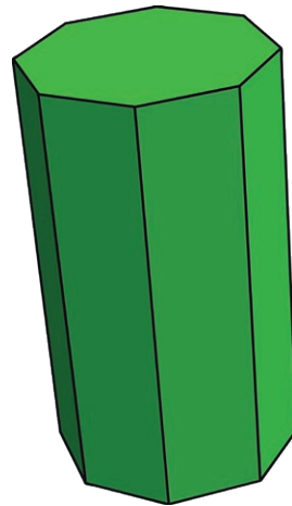
octagonal prism
