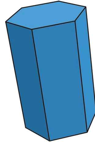
hexagonal prism
