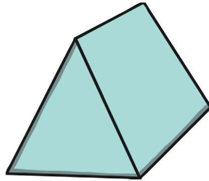
triangular prism
