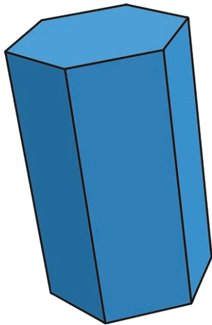
hexagonal prism
