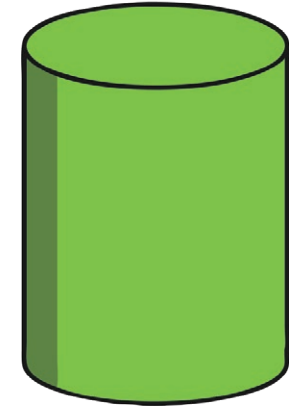
cylinder
