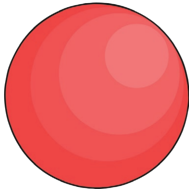
sphere
