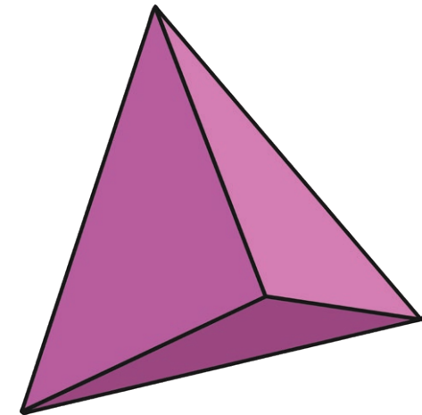
tetrahedron
