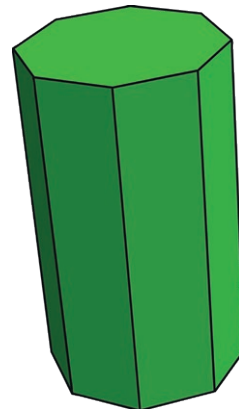
octagonal prism
