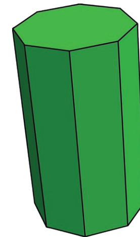
octagonal prism
