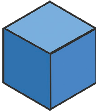
cube
