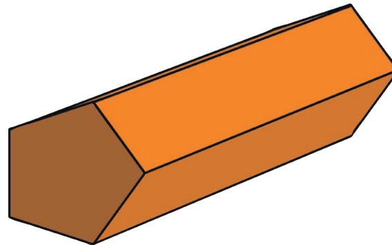
pentagonal prism
