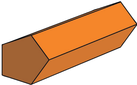
pentagonal prism
