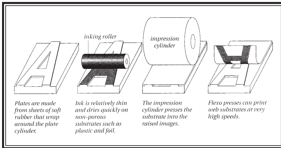
The flexographic printing process
