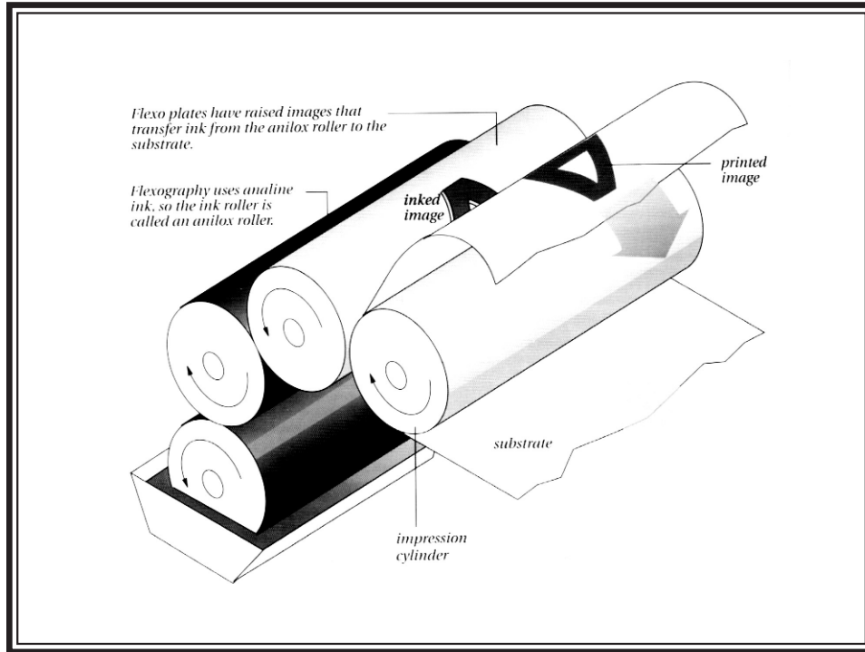
Schematic of single-color flexographic press
