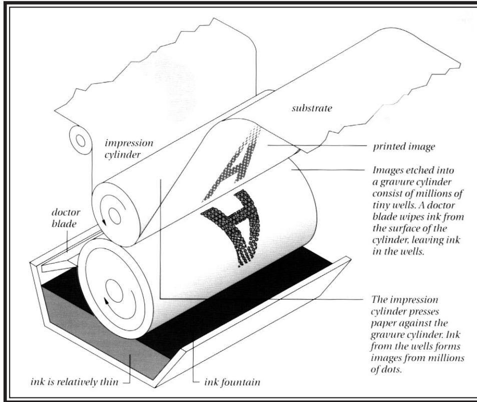
Schematic of single-color gravure press
