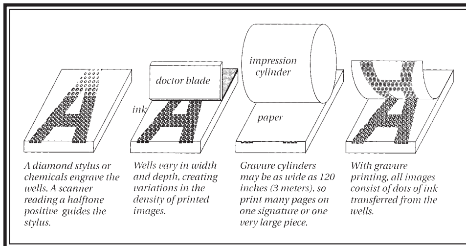
The gravure printing process
