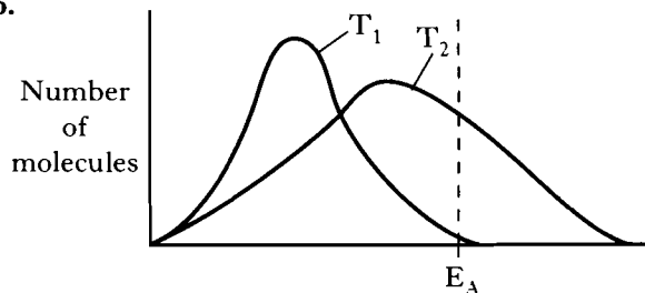
Kinetic energy of molecules
