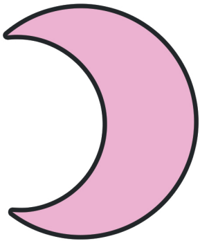
crescent
