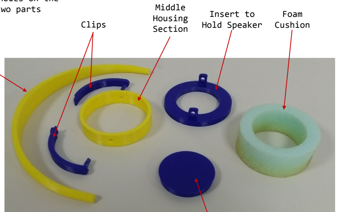
Speaker Insert
