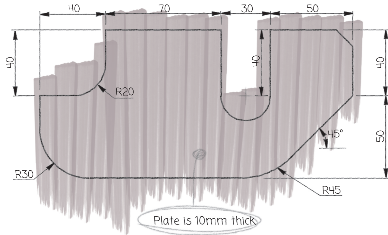
Orthographic preliminary sketch of bracket.
