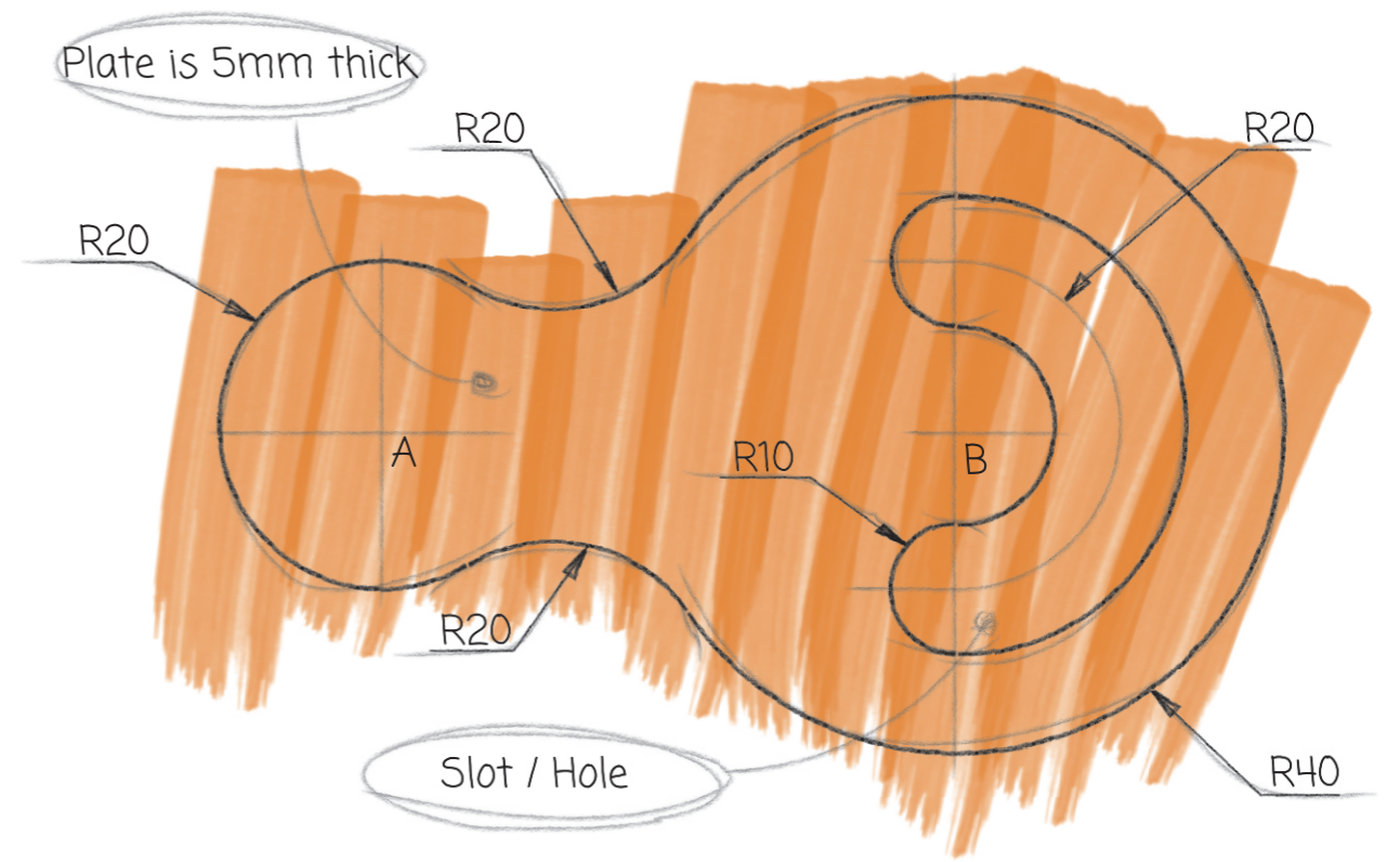
Orthographic preliminary sketch of bracket.
