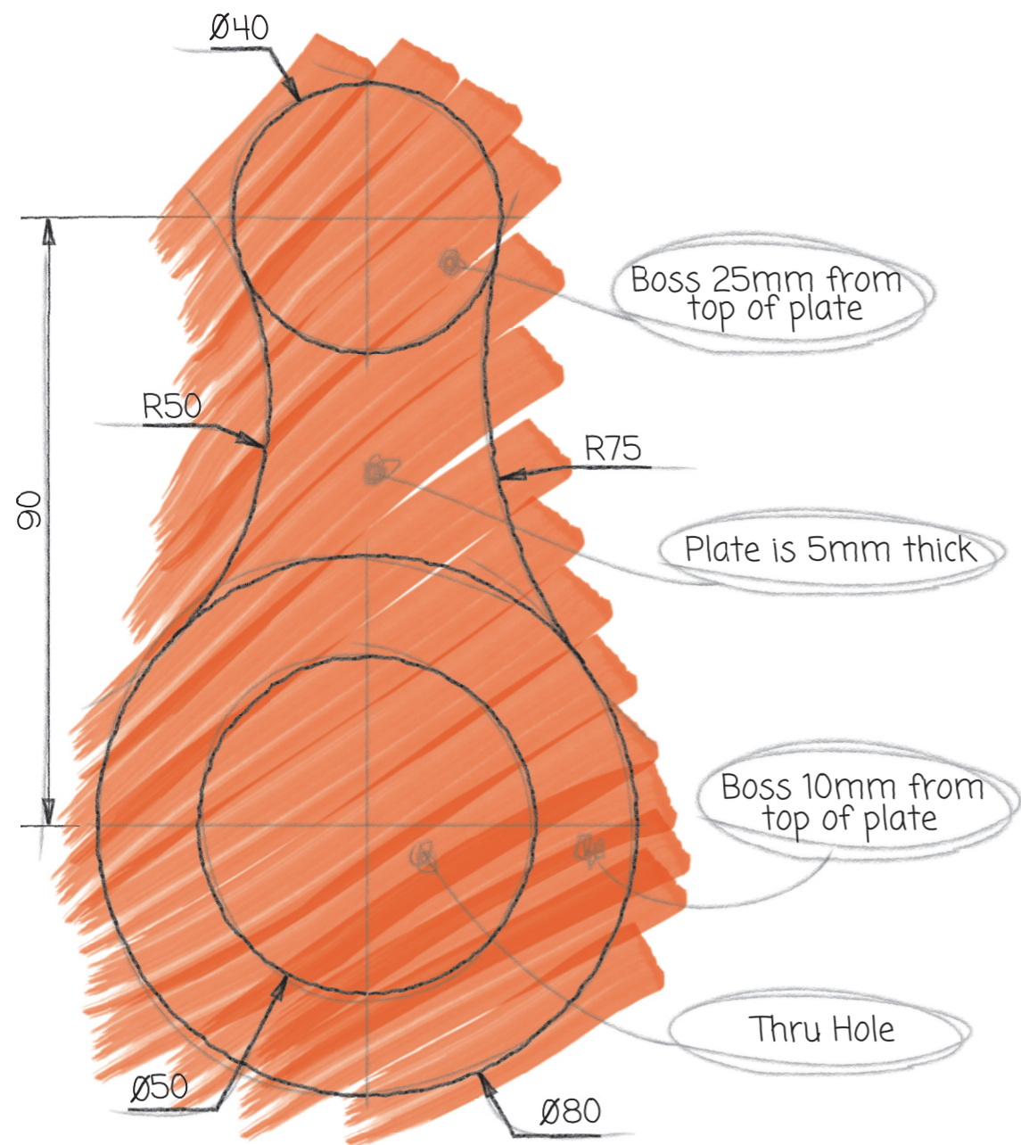
Orthographic preliminary sketch of bracket.
