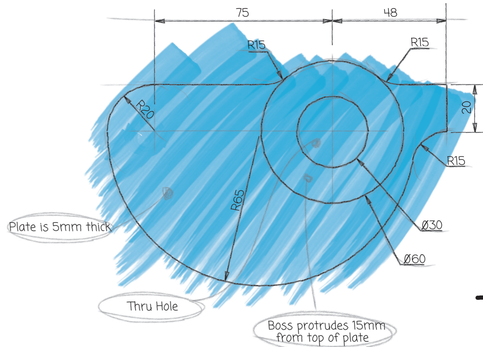
Orthographic preliminary sketch of bracket.
