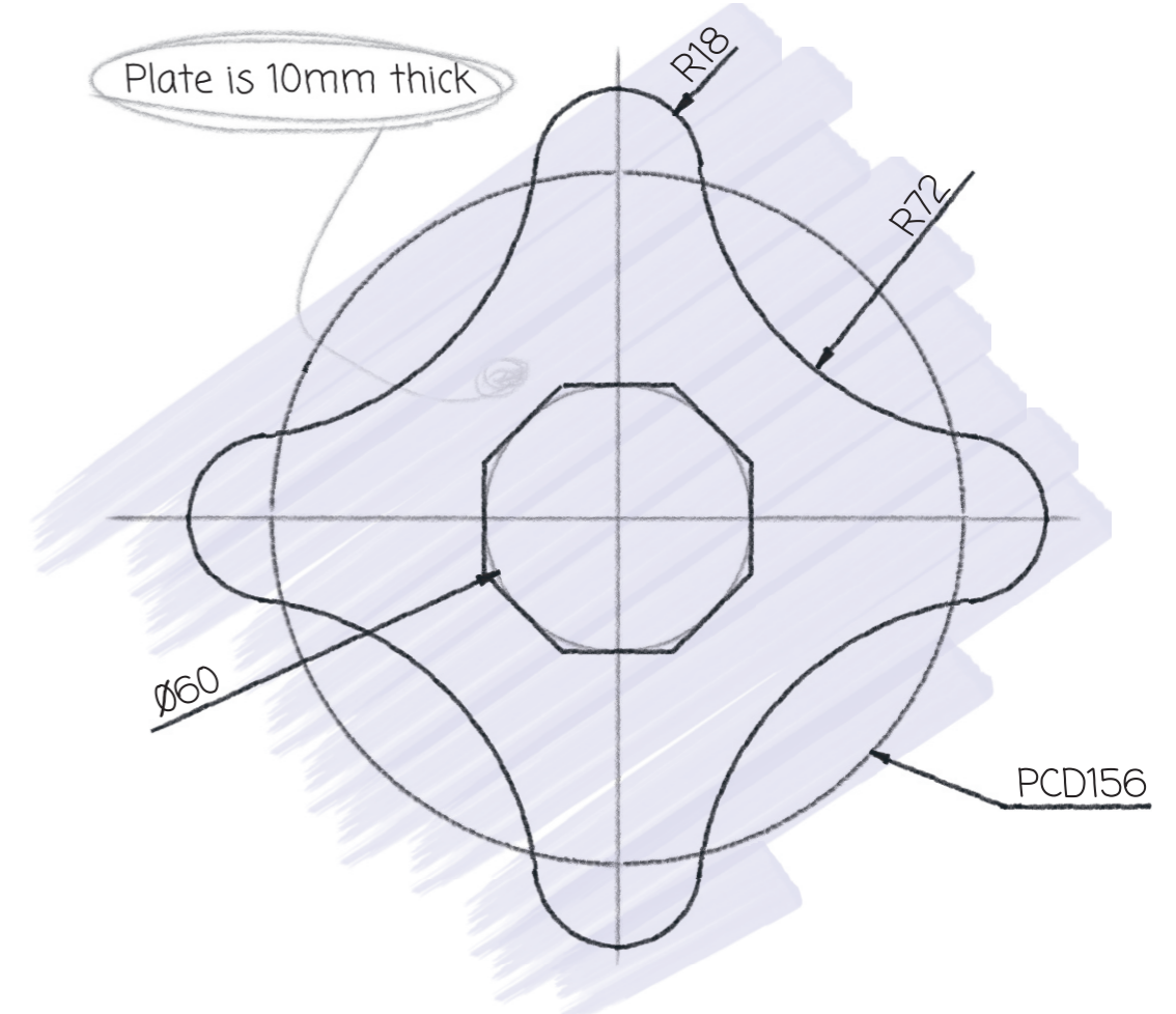
Orthographic preliminary sketch of bracket.
