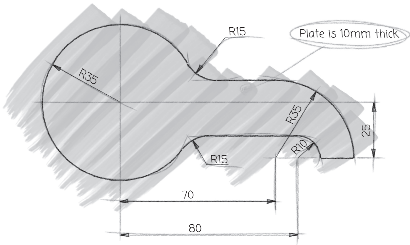
Orthographic preliminary sketch of bracket.
