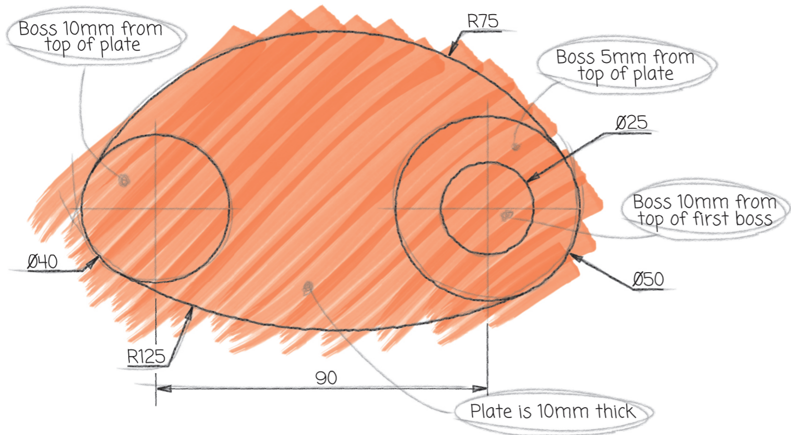
Orthographic preliminary sketch of bracket.
