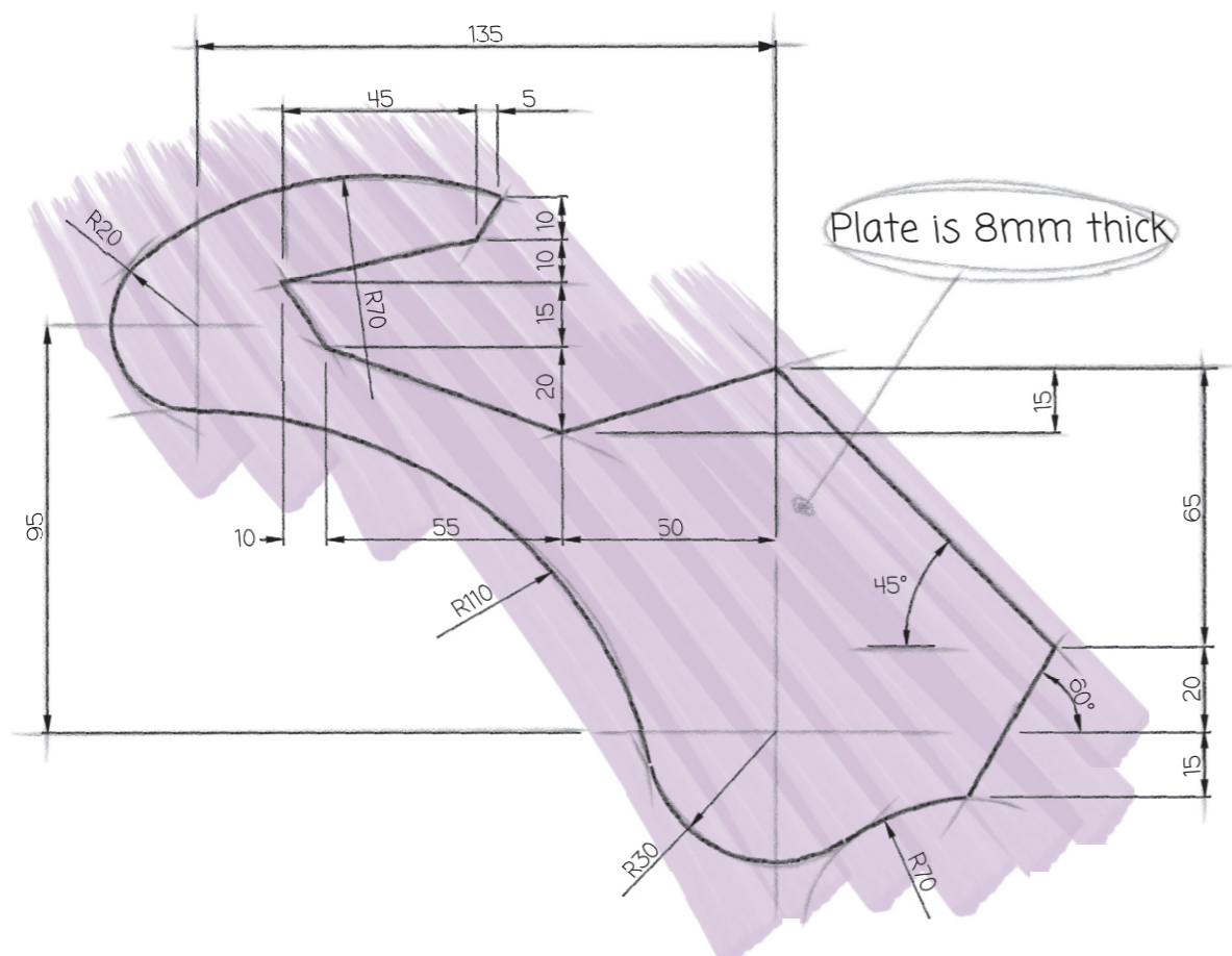
Orthographic preliminary sketch of bracket.
