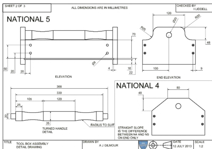
Orthographic Drawing
